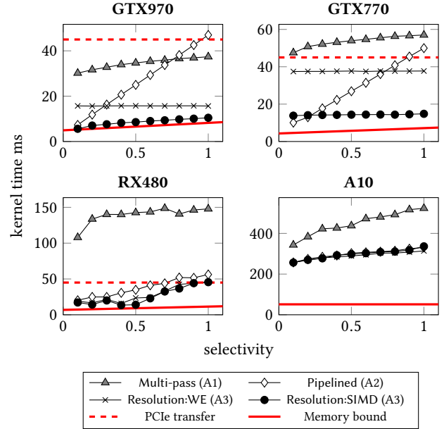
Figure 17: Projection query executed with different approaches. Integrating prefix sums into kernels allows fastest execution.
