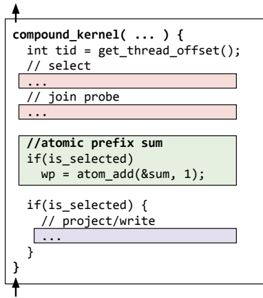
Figure 12: The compound kernel integrates all three pipeline phases into one kernel.
