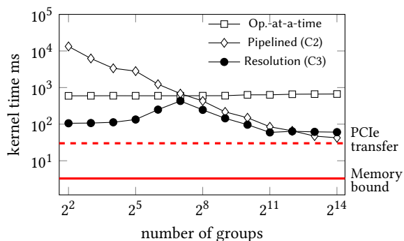
Figure 18: Performance of grouped aggregations.
