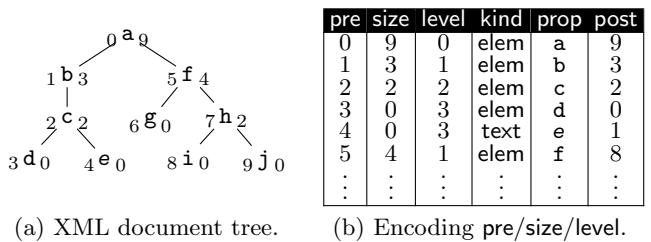
Fig. 1: XML document tree, annotated with \text{pre}(\cdot) and \text{size}(\cdot) information (left/right), and resulting tree encoding.
