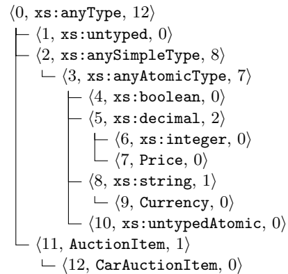
Fig. 8: Sample type hierarchy, annotated with pre(·) (left) and size(·) (right) numbers.
