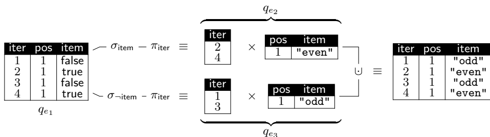
Fig. 3: Execution trace for loop-lifted execution of Query Q_1 . Using textbook-style algebra operators, the loop-lifted sequence representation is maintained for all subexpressions (illustrated for subexpressions e_1 through e_3 ).
