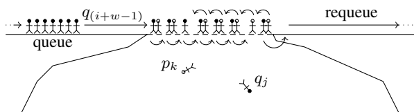
Figure 4. Lemming skyline: parallel BNL for FPGAs.
