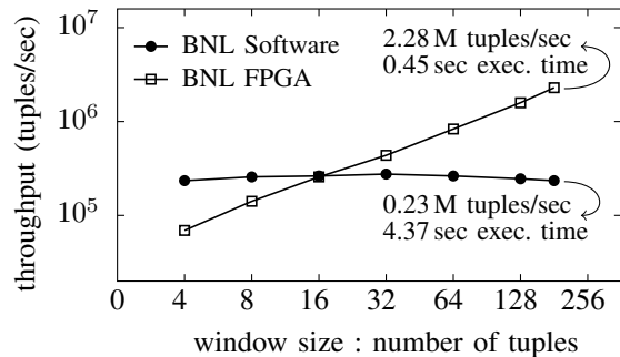
Figure 13. Randomly distributed dimensions \rightarrow tuples per second.
