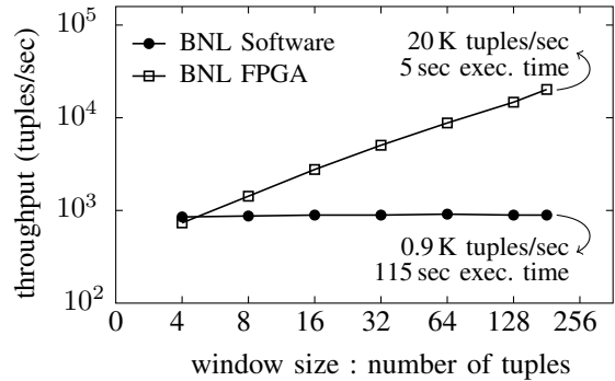
Figure 16. 15 dimensions (randomly distributed) → tuples per second.
