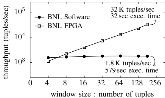
Figure 15. Anti-correlated dimensions → tuples per second.
