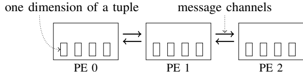
Figure 5. Working set items ( i.e. , tuples with several dimensions) are distributed over a pipeline of processing elements. Neighboring processing elements are connected via message channels.
