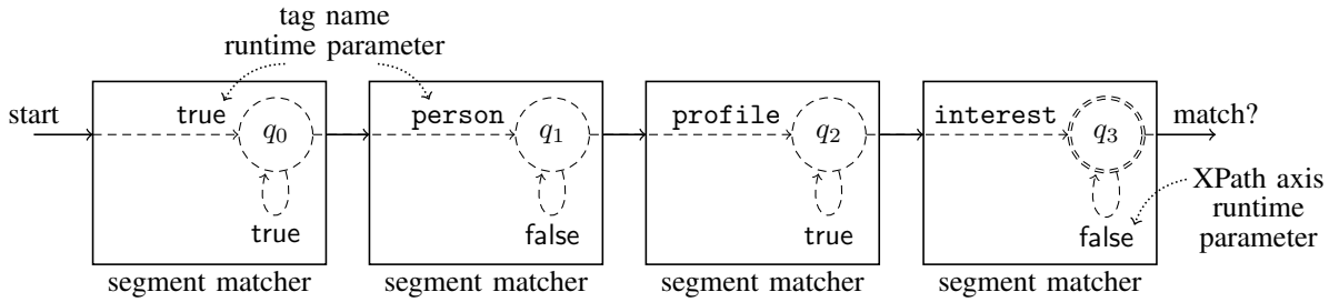
Fig. 3. Two-part “soft automaton” design for hardware-based XML projection in MXQuery/H . The FPGA configuration mechanisms are used to realize the static part of the automaton (drawn as solid lines), whereas all query-specific behavior is covered by the dynamic part (dashed lines) that can be parameterized at runtime.
